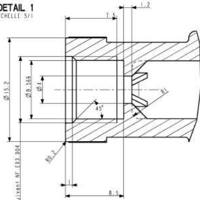
DETAIL 1 ECHELLE 5/1
